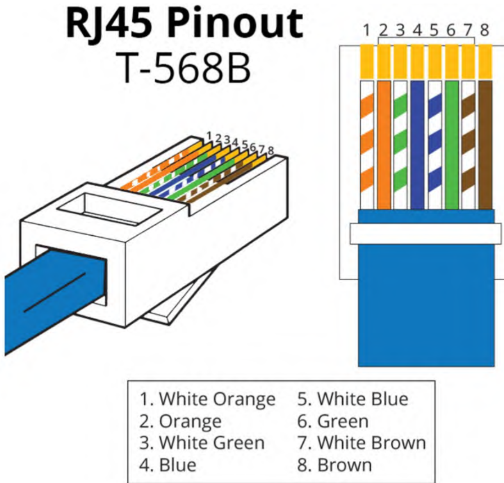
Figure 13 - RJ45 Ethernet Pinout
